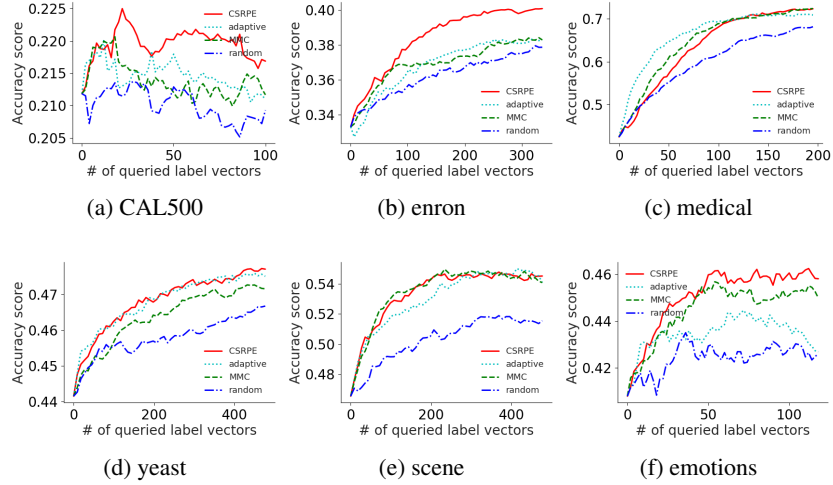
Fig. 7: CSMLAL results with Accuracy score \uparrow
